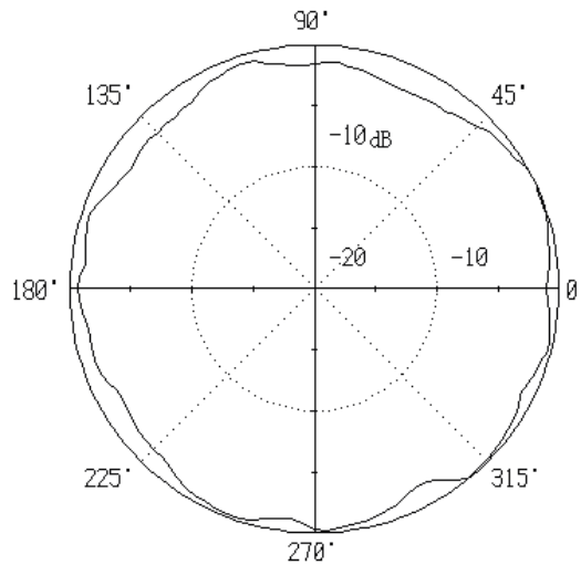
H Plane
