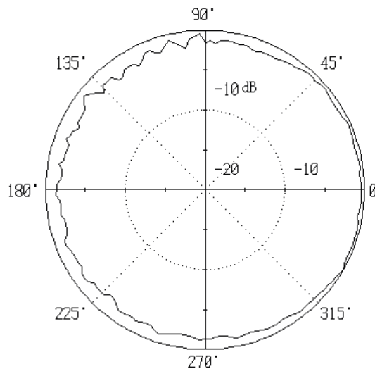
H Plane
